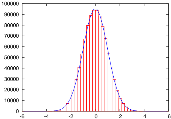
randn approximated with sum of 12 uniforms
