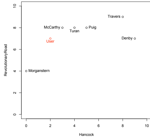
Figure 1: Plot of critics in a 2-dimensional review space for Hancock and Revolutionary Road . For the pair of films under consideration the Euclidean distance between two points provides a measure of how different two reviewers are.
