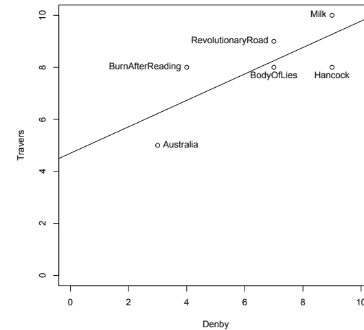
Figure 2: Plot of films in a 2-dimensional space defined by the ratings of David Denby and Peter Travers. The best fit straight line for these points is also plotted.
