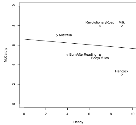
Figure 3: Plot of films in a 2-dimensional space defined by the ratings of David Denby and Todd McCarthy. The best fit straight line for these points is also plotted
