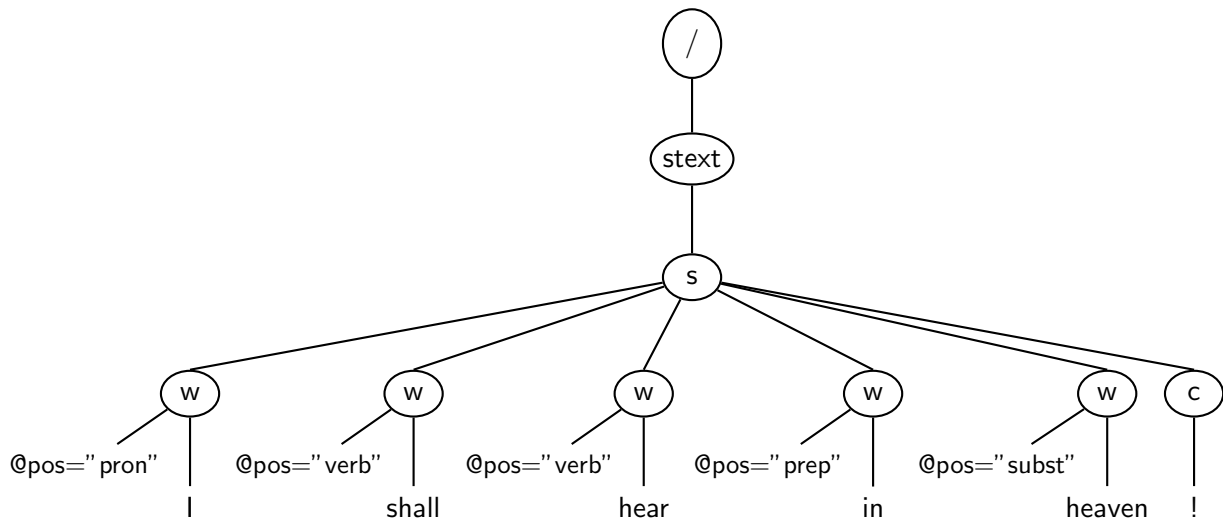
Figure 1: An XML tree
