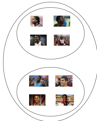
A set of sets of GB athletes
