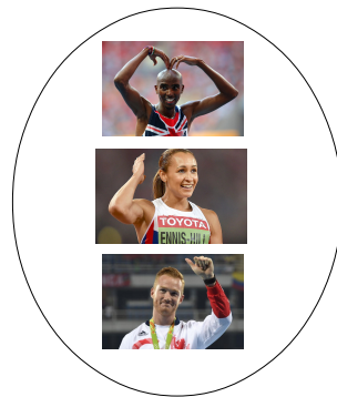
A set of GB athletes
