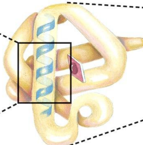
Polypeptide chain
