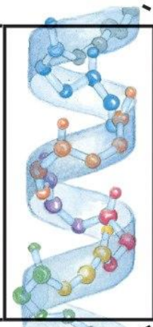
\alpha Helix
