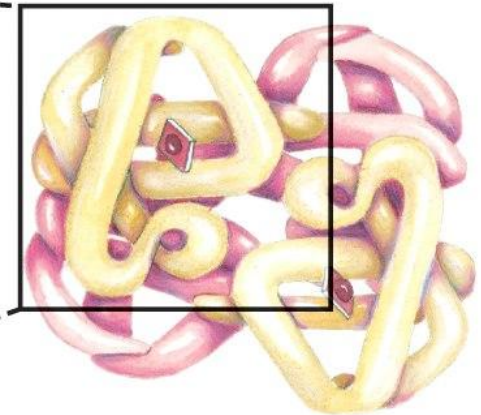
Assembled subunits
