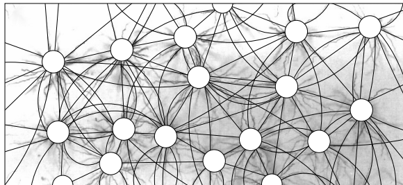
Integrate-and-fire / firing-rate model of the network
