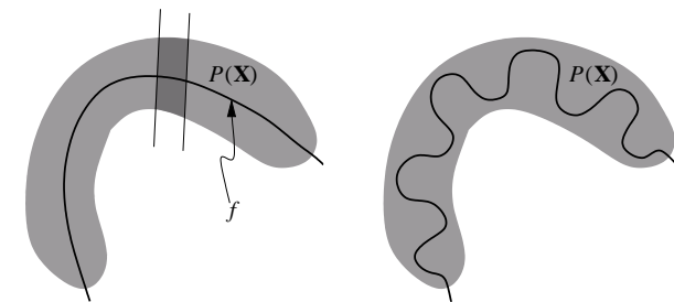
Principal curve
