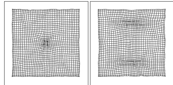
Gaussian distribution
