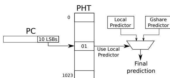
Figure 3: Tournament Branch predictor with a a 1024-entry PHT
