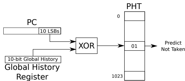
Figure 2: Gshare Branch predictor with a 10-bit GHR and a 1024-entry PHT
