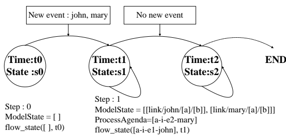
Figure 6: State Transition of the FWFL Workflow Engine
