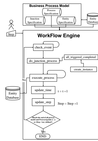
Figure 5: Flowchart of the FWFL Workflow Engine
