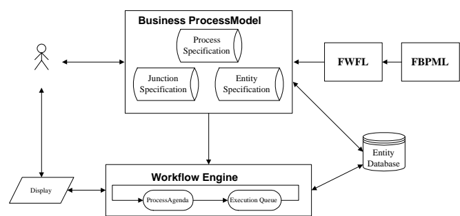
Figure 4: System Architecture of the FWFL Workflow Engine
