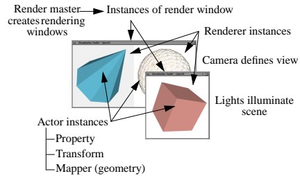
Figure 2 Graphics model
