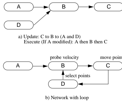
Figure 5 Network execution
