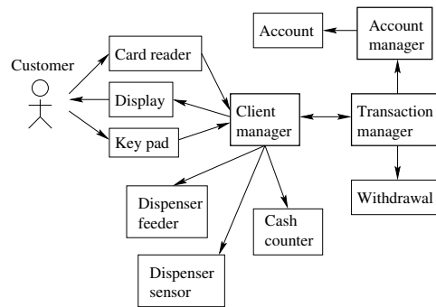
Figure 7: Interactions between design classes - part of design realisation
