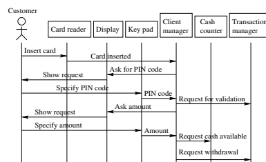
Figure 8: A sequence diagram for part of the realisation
