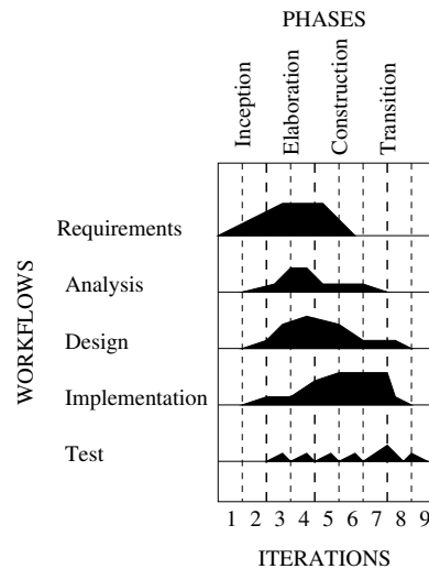
Figure 1: Phases in a cycle of the Unified Process
