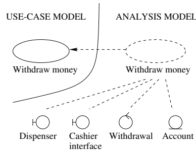
Figure 4: Analysis model for withdrawing money
