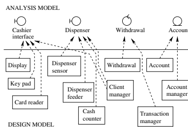
Figure 6: Design classes introduced for analysis classes
