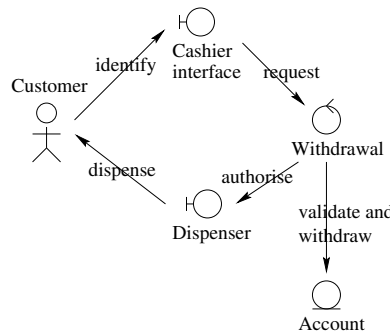
Figure 5: Collaboration model for withdrawing money
