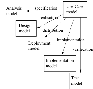
Figure 2: A series of models in the Unified Process
