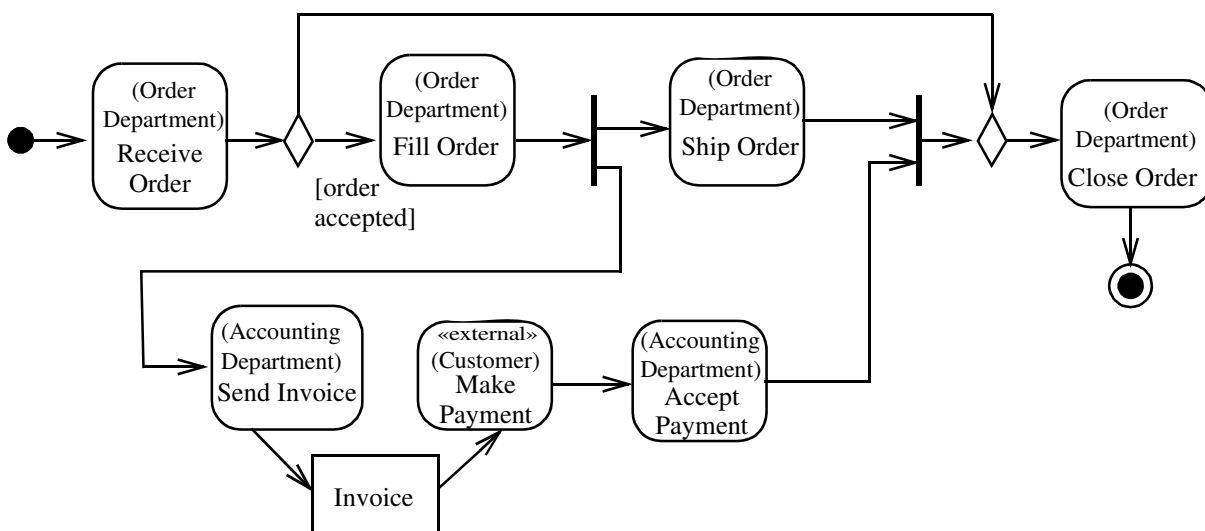
Figure 12.60 - Activity partition using annotation example
