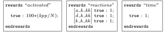
Figure 5: Reward structures for the cascade
