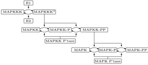
Figure 1: MAPK cascade pathway
