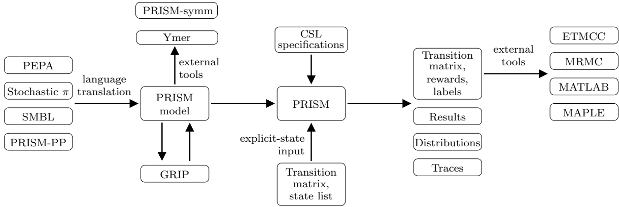
Figure 7: Language and tool connections for PRISM
