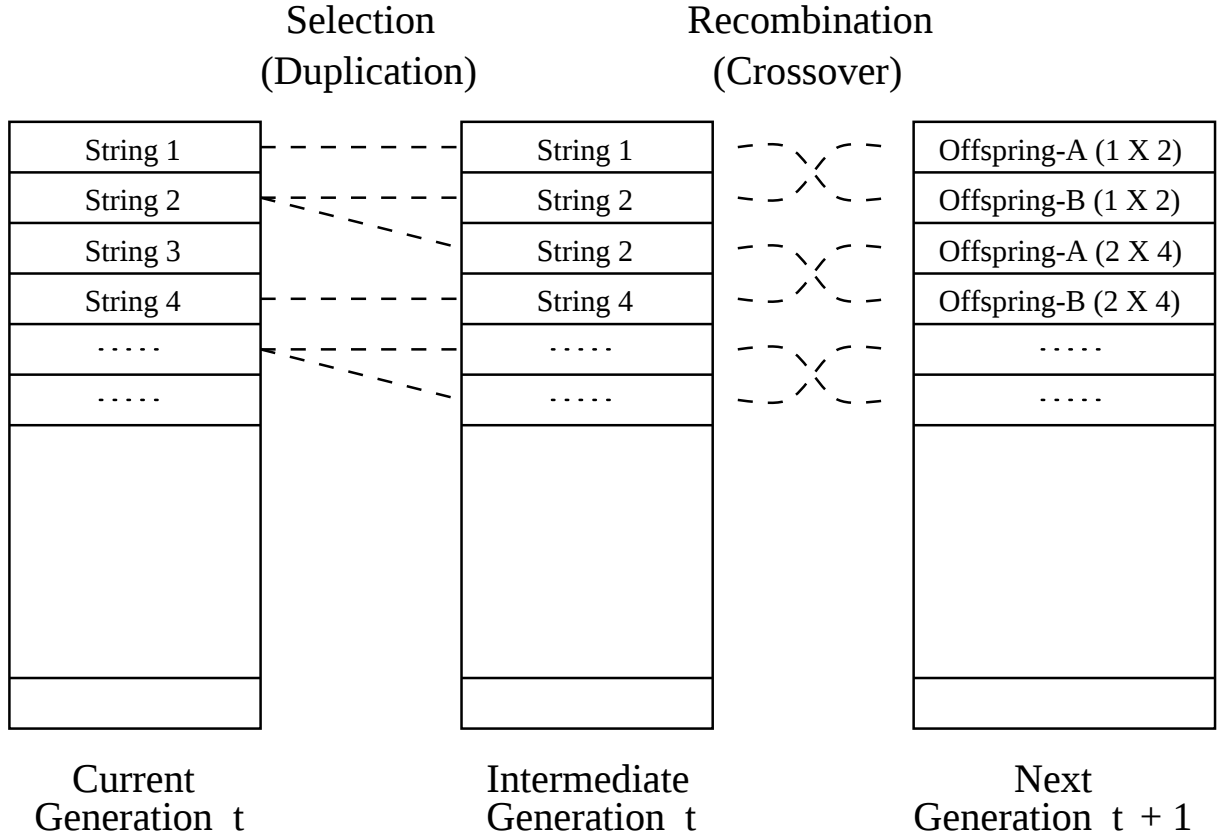
Figure 1: One generation is broken down into a selection phase and recombination phase. This figure shows strings being assigned into adjacent slots during selection. In fact, they can be assigned slots randomly in order to shuffle the intermediate population. Mutation (not shown) can be applied after crossover.
