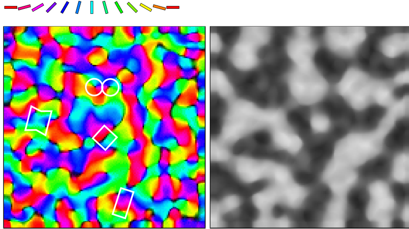
OR preference & selectivity
