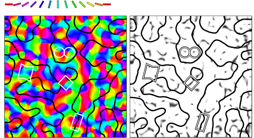
OR preference & OD boundaries
