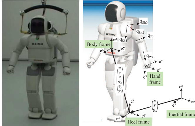
Fig. 1. ASIMO humanoid robot (left) and kinematic model used for whole body motion control (right) [15]. In our experiments 22 upper body degrees of freedom were used ( 2 \times 7 DOF arms, 2 DOF head, 6 DOF torso), with the heel frame fixed.
