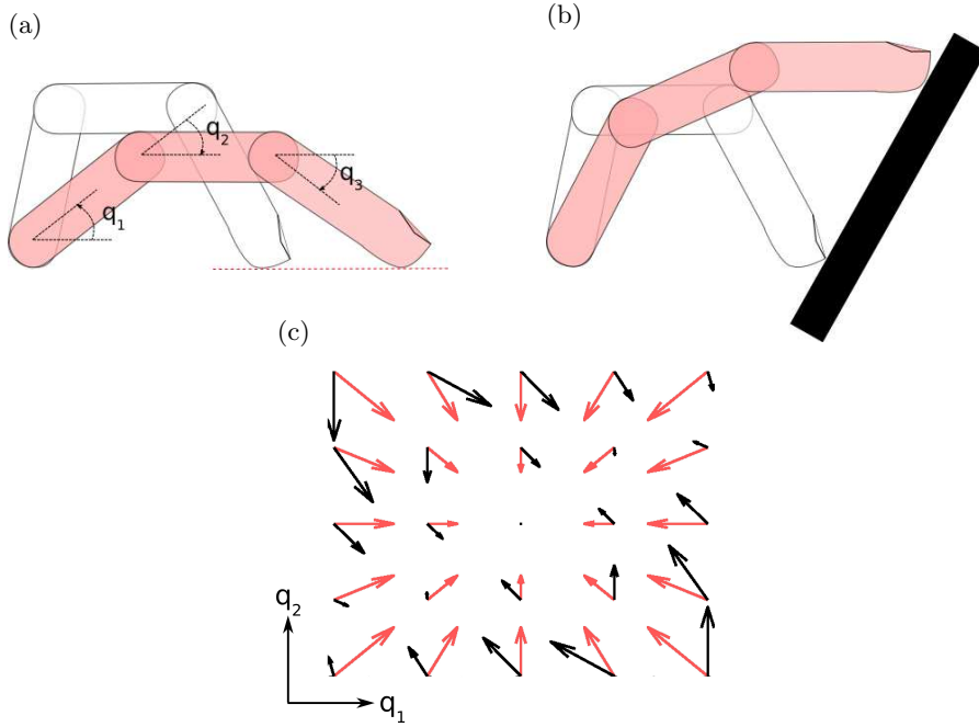
Fig. 2. Illustration of two apparently different behaviours from the same policy: (a) unconstrained movement (b) movement constrained by an obstacle (black box) (c) vector field visualisation of the unconstrained (red) and constrained (black) policy for two of the finger joints as a function of their angles.
