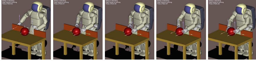
Fig. 9. Example constrained trajectory used as training data in the ball-reaching experiment. Starting with hands at the sides, the demonstrator robot reaches between the barriers to get the ball. Note that the width of the gap in the barriers was randomly altered for each trajectory recorded.
