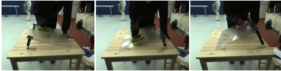
Fig. 12. Human wiping demonstrations on surfaces of varying tilt and rotations. The ASIMO stereo vision system was used to track the 3-D coordinates of the sponge (coloured rectangles show the estimated position). Tilts of \pm 16^\circ and +27^\circ about the x -axis are shown.
