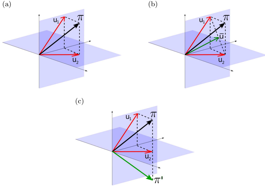
Fig. 3. Illustration of the effect of constraints on the unconstrained policy, the averaging effect of direct regression and the degeneracy problem. (a) Two constraints applied to the policy \pi result in projected observations \mathbf{u}_1, \mathbf{u}_2 . (b) Direct regression results in averaging of the two movements \bar{\mathbf{u}} in a way that cannot explain the observations. (c) Two policies \pi, \pi' that both may be constrained in such a way as to produce the observation \mathbf{u}_2 .
