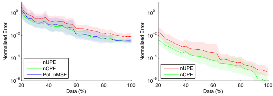
Fig. 7. Learning performance on the quadratic potential (31) with varying data set sizes for the alignment approach (left) and the inconsistency approach (right). Normalised CPE and UPE versus data set size as a percentage of the full K = 40 trajectories of length N = 40 are shown. For the alignment approach the normalised error in the potential is also plotted.
