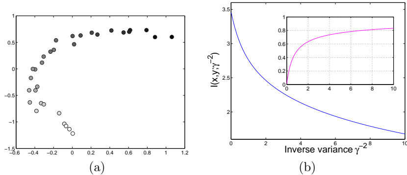
Figure 1: (a): training data, M = 50 , |\mathbf{x}| = 2 . (b): change of \tilde{I}(\mathbf{x}, \mathbf{y}; \gamma^2) with an increase of the inverse variance \gamma^{-2} for Squared Exponential kernels, |\mathbf{y}| = 1 . Insert : Residuals \text{res}(\gamma^{-2}) \stackrel{\text{def}}{=} (M - \lambda_1(\mathcal{K}_\gamma))/M as a function of \gamma^{-2} .
