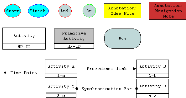
Figure 3. FBPML Notation
