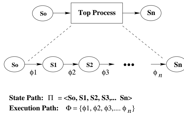
Figure 4. Execution Path for Processes
